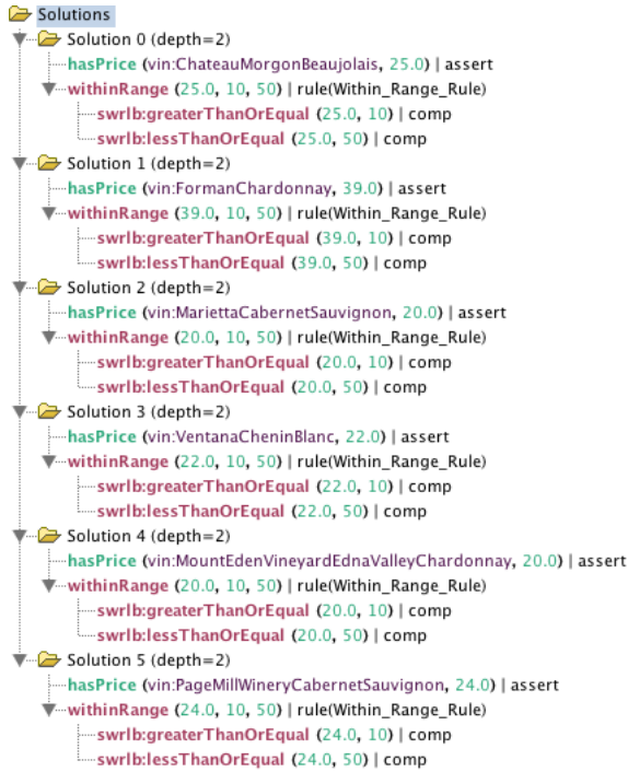
Fig. 3. Price range query trace
